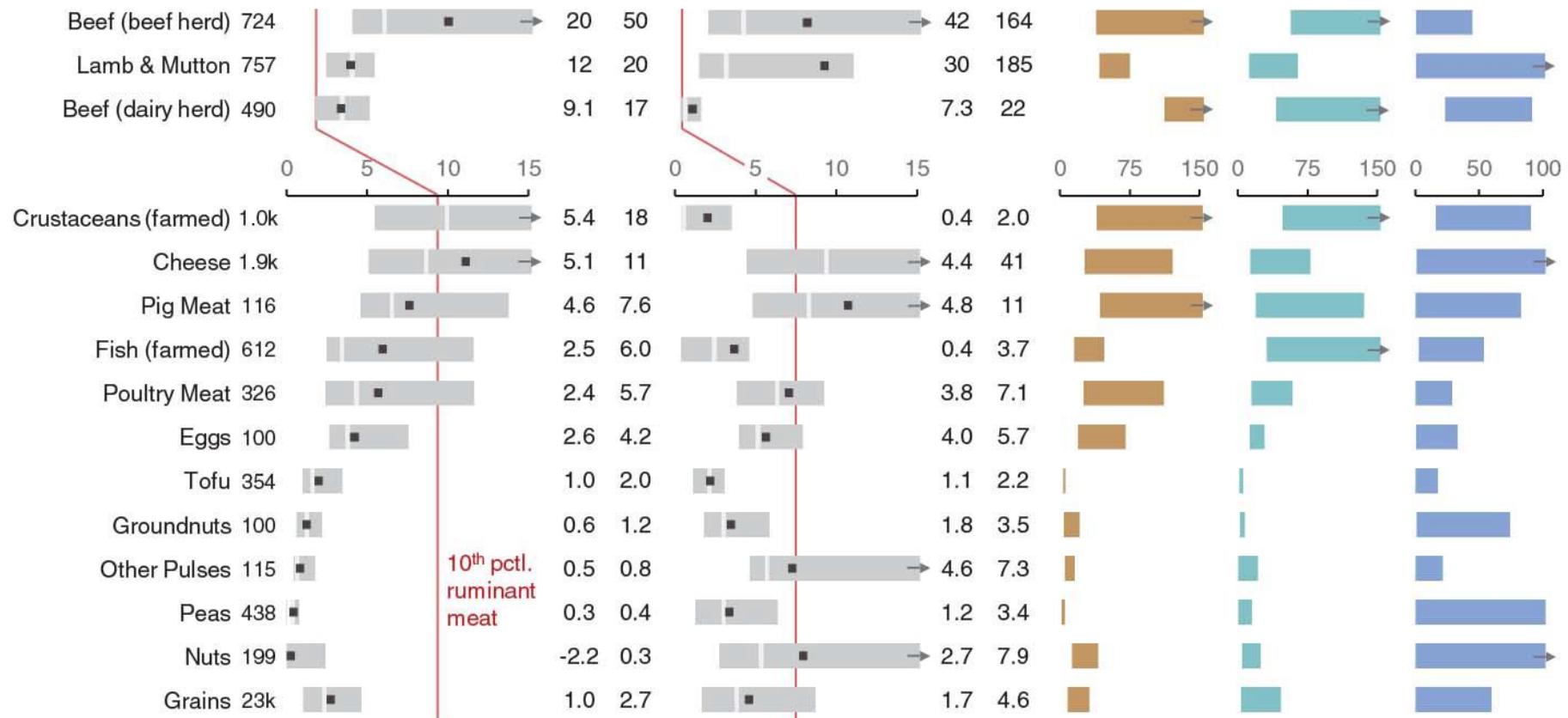
Estimated global variation in GHG emissions, land use, terrestrial acidification, eutrophication, and scarcity-weighted freshwater withdrawals, within and between 40 major foods 1
